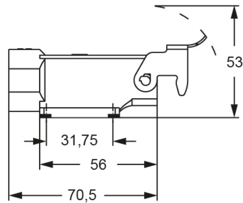
Catalogue drawings
