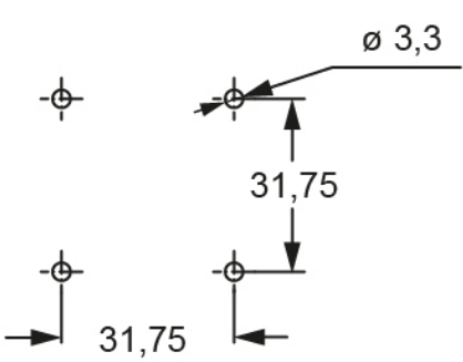
Catalogue drawings
